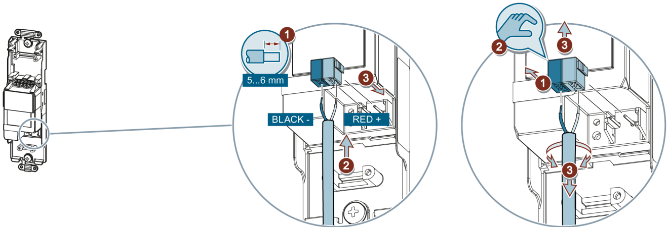
Fig. 4: Solar protection actuator RL 524D23, 2 x 6 A DC
